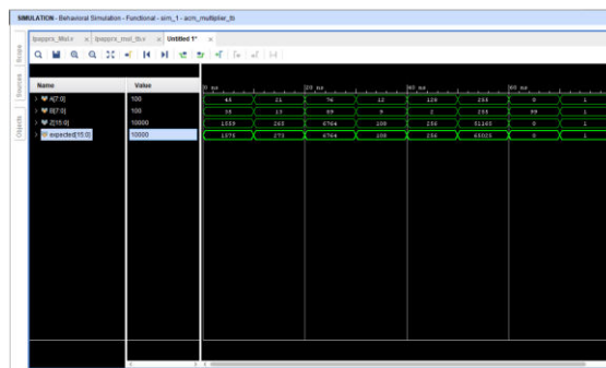
Fig: simulation of the design for various inputs is verified for the proposed design.
